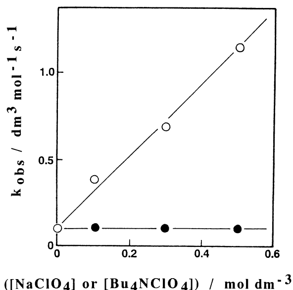
Fig. 1. Plots of k_{\text{obs}} vs. [\text{NaClO}_4] ( \circ ) or [\text{Bu}_4\text{NClO}_4] ( \bullet ) for the one-electron reduction of \text{Cl}_4\text{Q}^{\cdot-} ( 5.0 \times 10^{-5} \text{ mol dm}^{-3} ) by BNAH in deaerated MeCN at 298 K.
